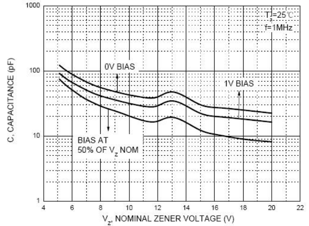
Typical Capacitance
