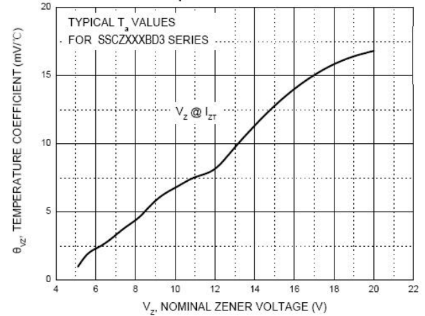
Temperature Coefficients
